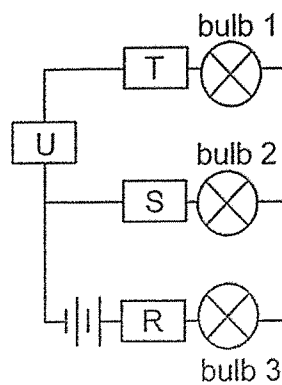
circuit B
