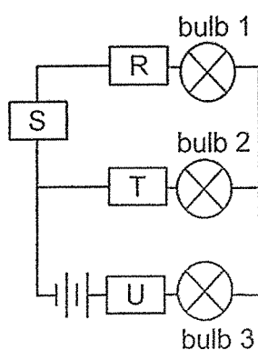
circuit A
